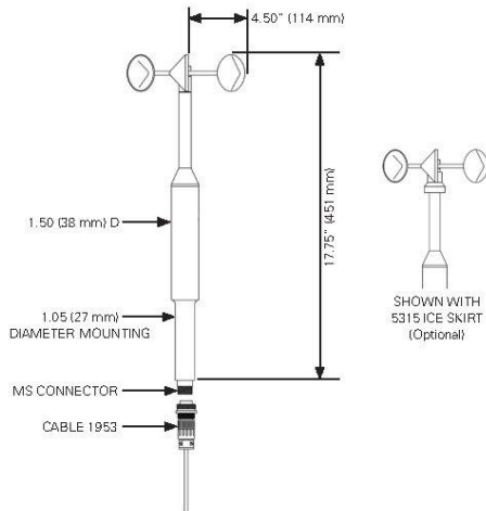
010C Wind Speed Sensor
